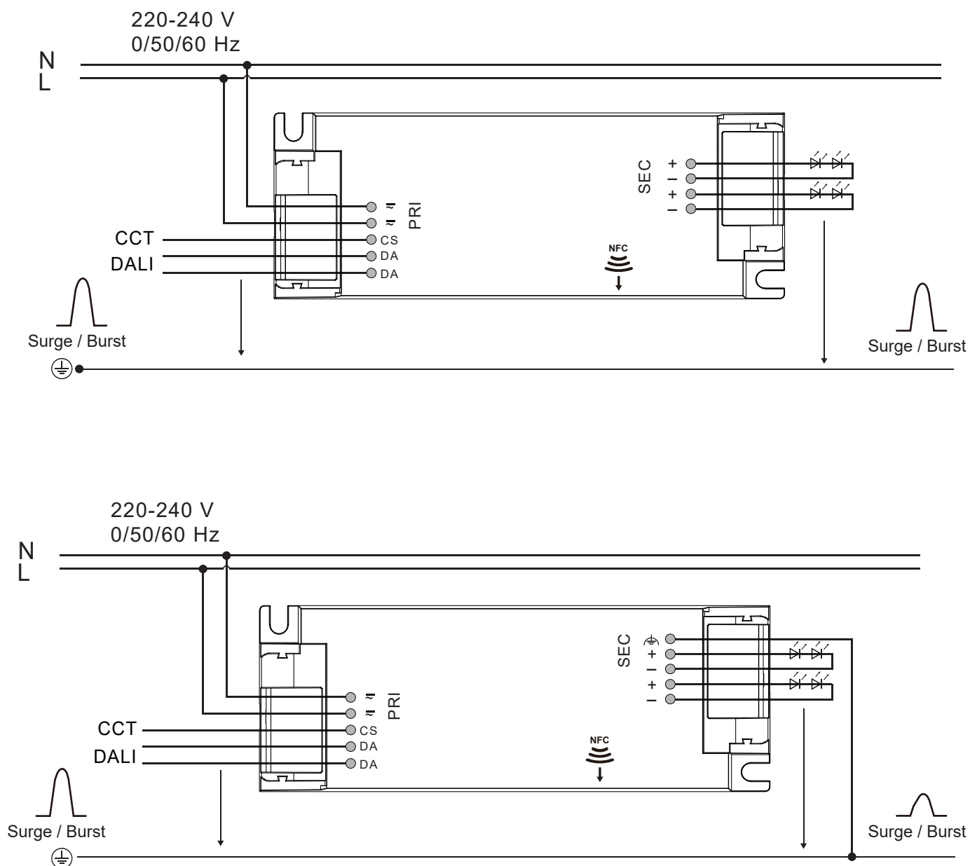
Figure: Voltage peaks for LED driver without earthing (Above) and with earthing (Below)
